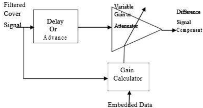
Fig. 4 Difference signal component generator
