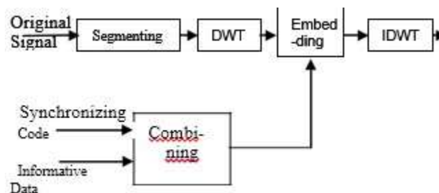
Fig. 4 DWT watermark embedding
