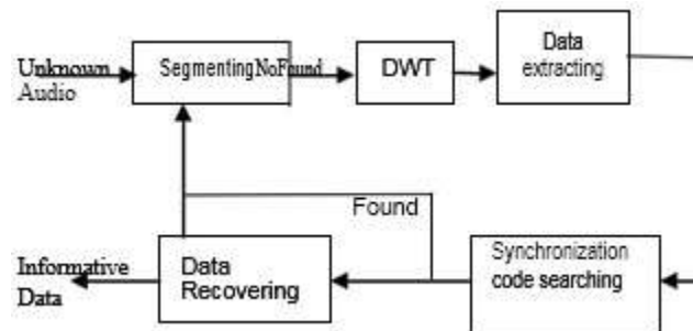
Fig. 5 Watermark Extraction
