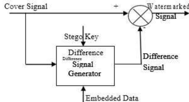
Fig. 3 Block Diagram of Embeddor
